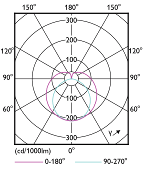
Light Distribution Diagram - 12T5HE/COR/34-5CCT/MF16/G 25/1
