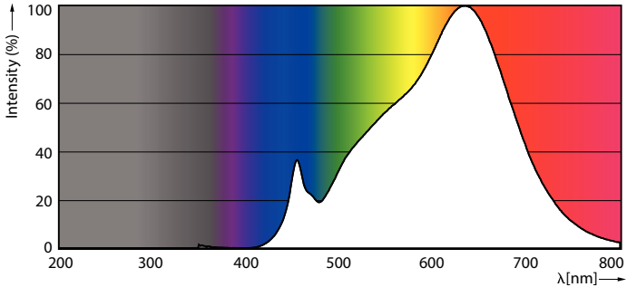
Spectral Power Distribution Colour - 14PAR38/EXPERTCOLOR/ F25/927/P/D/T20/JA8
