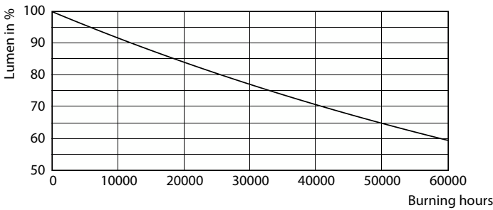
Lumen Maintenance Diagram - 14PAR38/EXPERTCOLOR/ F25/927/P/D/T20/JA8
