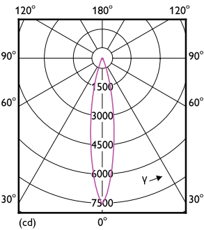
Light Distribution Diagram - 14PAR38/EXPERTCOLOR/ F25/927/P/D/T20/JA8
