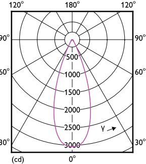
Light Distribution Diagram - 14PAR38/EXPERTCOLOR/ F40/927/P/D/T20/JA8
