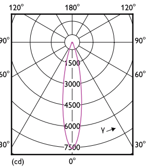
Light Distribution Diagram - 14PAR38/EXPERTCOLOR RETAIL/F25/930/P/D/B
