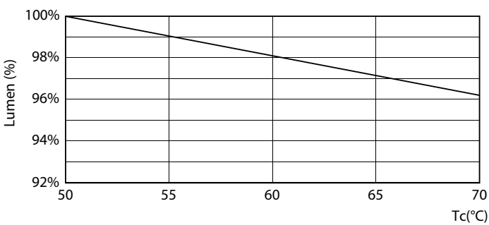
MC LEDtube 16W 60K LumenVsTc
