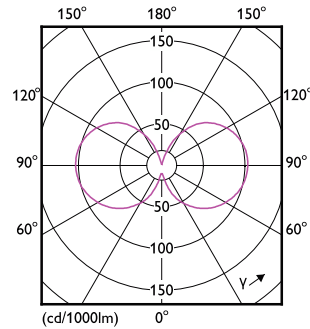
Light Distribution Diagram - 15GC/LED/830/ND E26 BB 6/1
