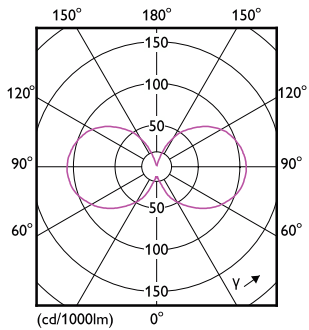
Light Distribution Diagram - 2.3BA11/PER/UD/CL/G/E12/WGD 6/3PFT20
