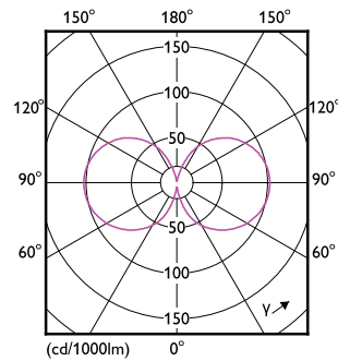
Light Distribution Diagram - 25GC/LED/840/ND E26 BB 6/1
