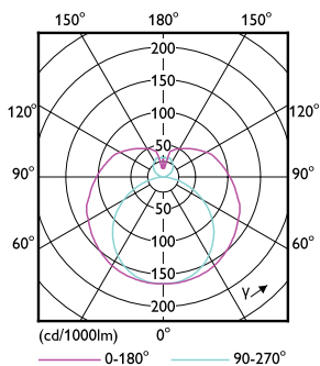
Light Distribution Diagram - 28T8/COR/96-835/IF40/G/FA8 10/1
