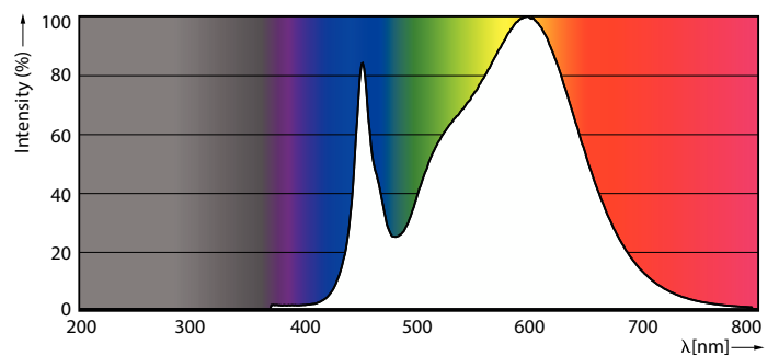
Spectral Power Distribution Colour - 28T8/COR/96-835/IF40/G/FA8 10/1
