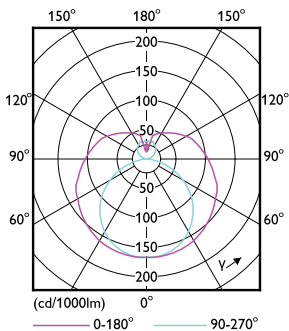
Light Distribution Diagram - 28T8/COR/96-840/IF42/G/FA8 10/1
