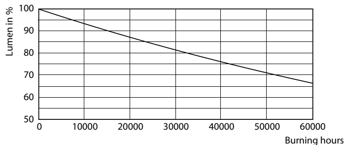
Lumen Maintenance Diagram - 28T8/COR/96-840/IF42/G/FA8 10/1
