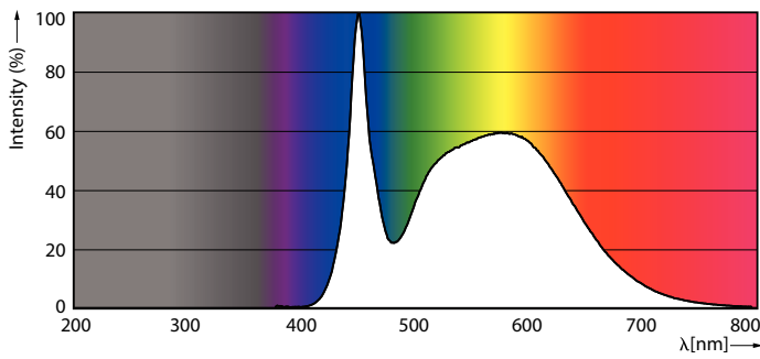
LEDTForce LS 450W Corncob EX39 850-POC
