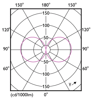
Light Distribution Diagram - 45GC/LED/830 EX39 BB 6/1
