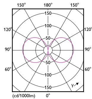
Light Distribution Diagram - 45GC/LED/850 EX39 BB 6/1
