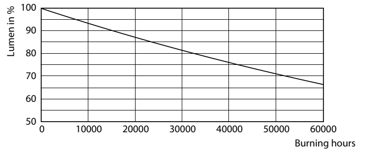
Lumen Maintenance Diagram - 45GC/LED/850 EX39 BB 6/1
