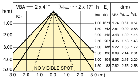
SDBE_LEDspotL_0147-Beam diagram
