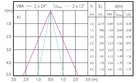
LEDSpots MR16 7W 940 460lm 25D
