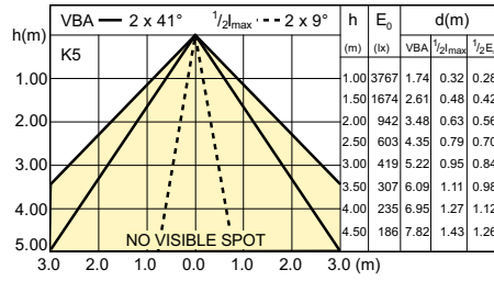
LEDspot 7-35W MR16 GU5.3 4000K 530lm 15D
