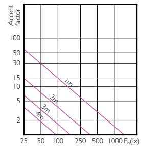
LEDSpots MR16 7W 930 460lm 35D
