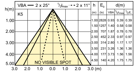
LEDspot 7-50W MR16 GU5.3 2700K 420lm 24D
