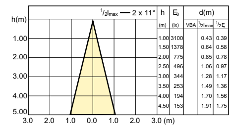
SDBE_LEDspotL_0117-Beam diagram
