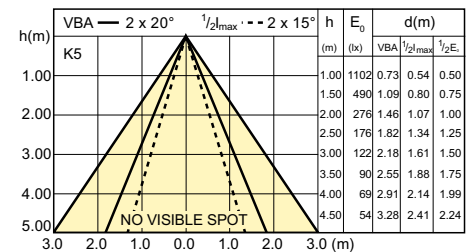
SDBE_LEDspotL_0130-Beam diagram
