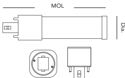
G24d/GX24d (2-pin)
