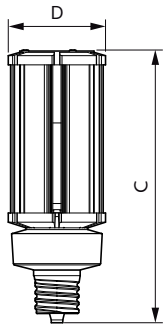
Corn lamp LED Gen2 54W EX39 850 CL
