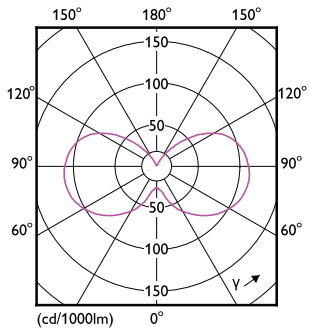
Light Distribution Diagram - 5B11/PER/UD/CL/G/E26/WGD 6/3PF T20
