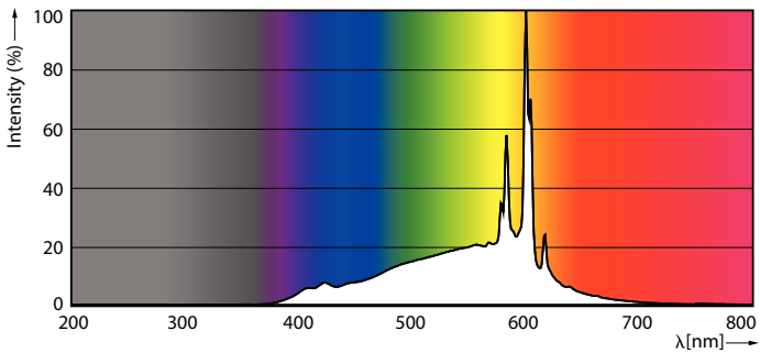
Spectral Power Distribution Colour - 5BA11/PER/UD/CL/G/E12/WGD 6/3PF T20
