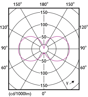
Light Distribution Diagram - 5BA11/PER/UD/CL/G/E12/WGD 6/3PF T20
