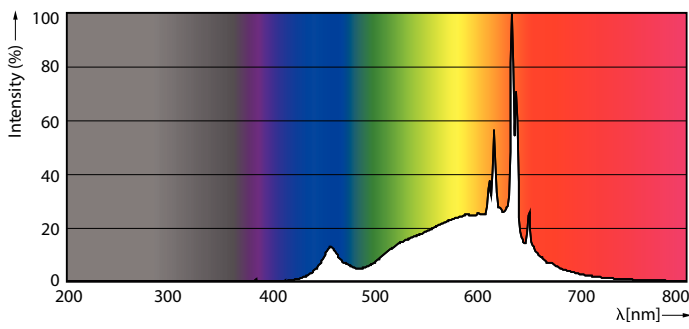
LEDbulb 45W E26 R20 927 Frosted
