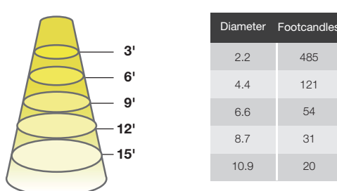
14PAR38DIM/9CCTS/BAS 40° 2700K
