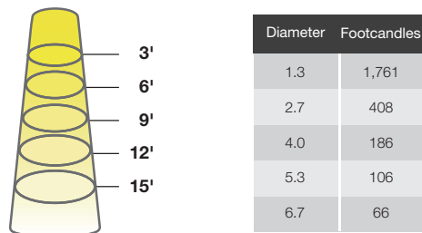
9PAR30SNDIM/9CCTS/BAS 25° 2700K
