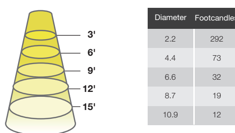
9PAR30SNDIM/9CCTS/BAS 40° 2700K
