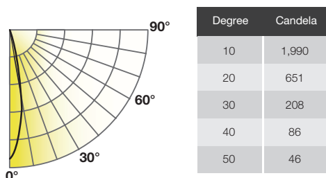
14PAR38DIM/9CCTS/BAS 25° 2700K
