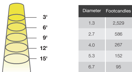
14PAR38DIM/9CCTS/BAS 25° 2700K
