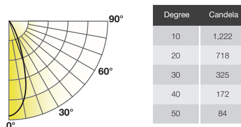
14PAR38DIM/9CCTS/BAS 40° 2700K
