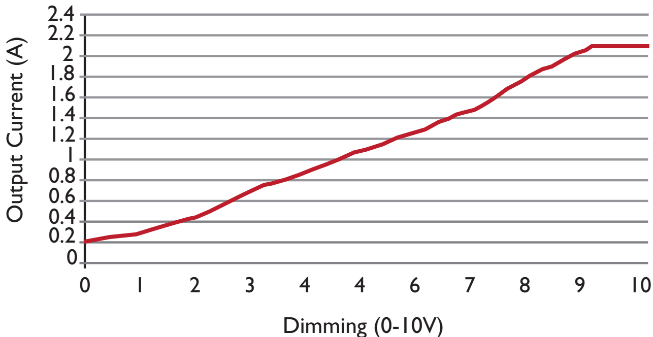
Output Current v.s. Dimming
