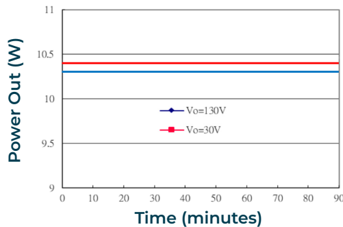
Constant output power performance over full 90 minutes run-time
