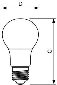
Bulb A19 Green 120V 5.5W-40W 2700K E26 N
