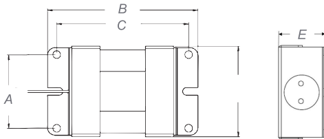
Battery Bracket
