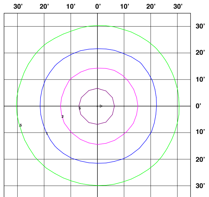
55W PARKING 15'
