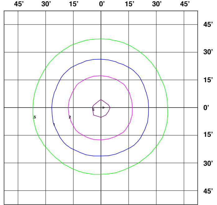
70W PARKING 20'
