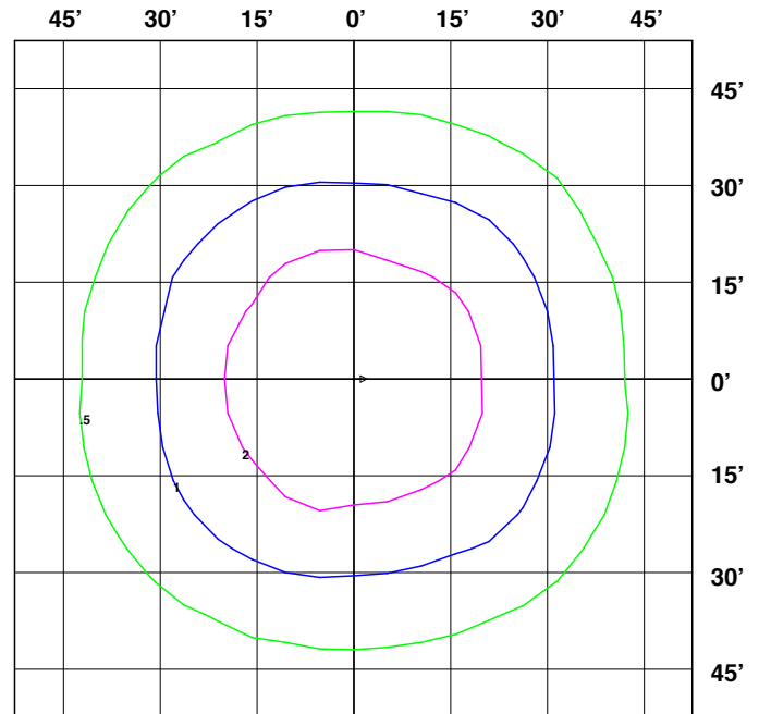
100W PARKING 25'
