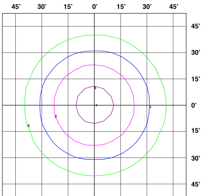
100W CANOPY 25'
