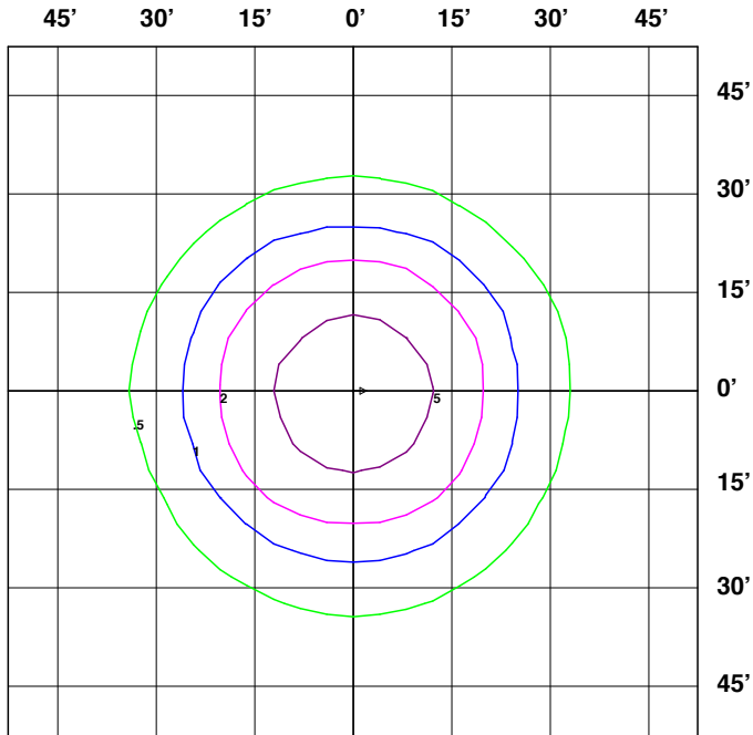
70W CANOPY 20'
