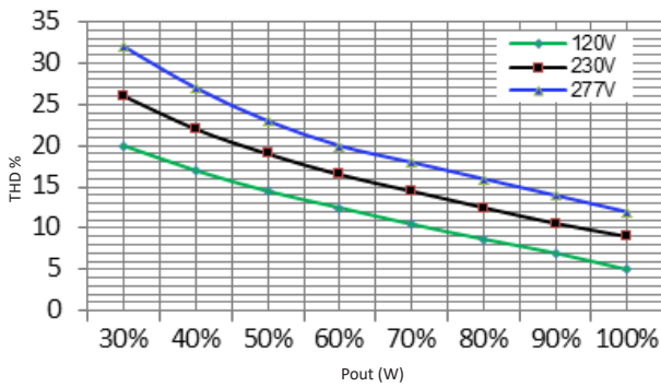
THD vs. Pout
