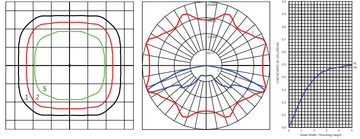
EALP Type VS - Symmetric High Angle 67,600 Lumens, 5000K (EALP03_Q5SH750__IES)
