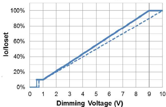
I_o/I_{o\text{set}} vs. Dimming Voltage
