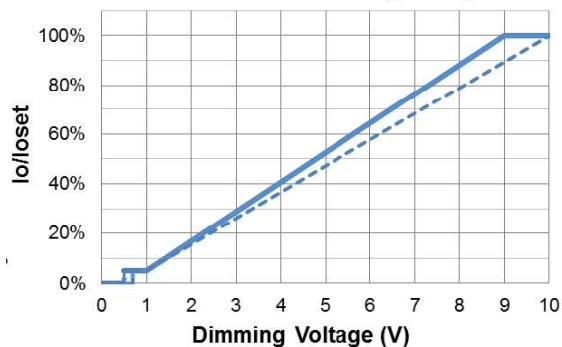
I_o/I_{o\text{set}} vs. Dimming Voltage
