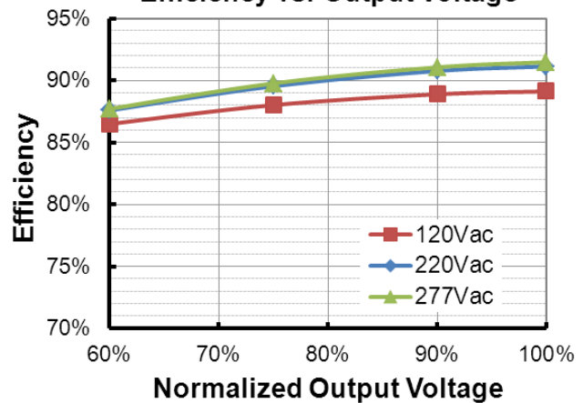
EUD-096S105DTL (I o =1050mA) Efficiency vs. Output Voltage
