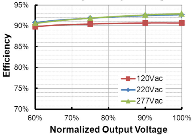
EUD-096S070DTL (I o =450mA) Efficiency vs. Output Voltage
