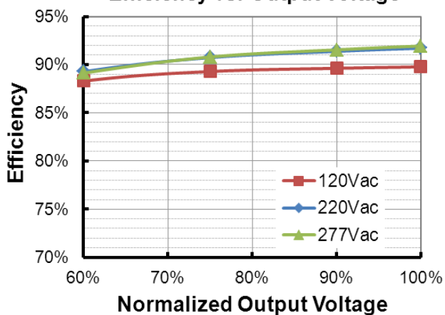
EUD-096S210DTL (I o =1400mA) Efficiency vs. Output Voltage
