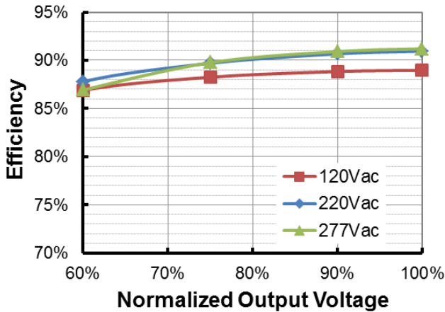
EUD-096S215DTL (Io=1750mA) Efficiency vs. Output Voltage
