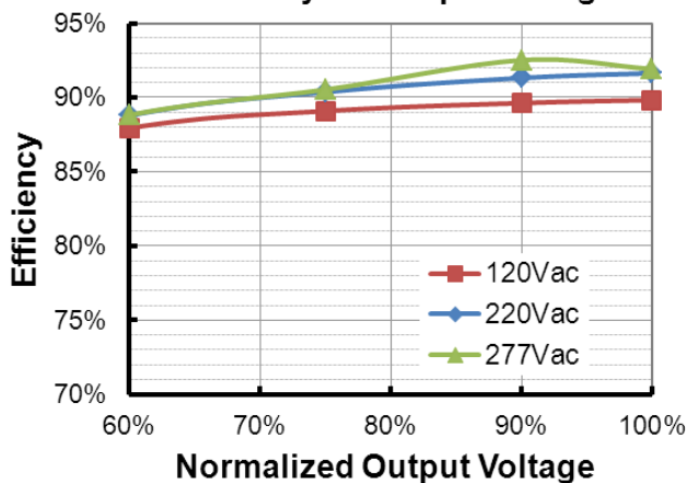
EUD-096S350DTL (Io=2450mA) Efficiency vs. Output Voltage
