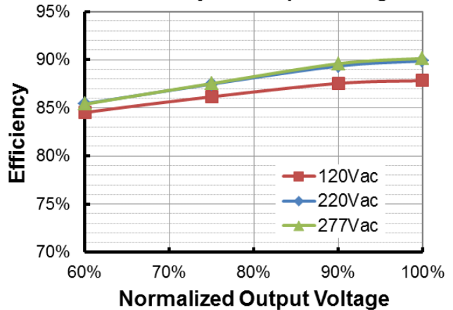
EUD-096S215DTL (Io=2150mA) Efficiency vs. Output Voltage
