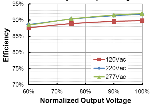
EUD-096S070DTL (I o =700mA) Efficiency vs. Output Voltage
