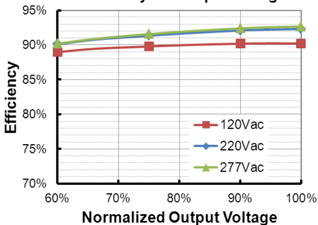
EUD-096S105DTL (I o =700mA) Efficiency vs. Output Voltage
