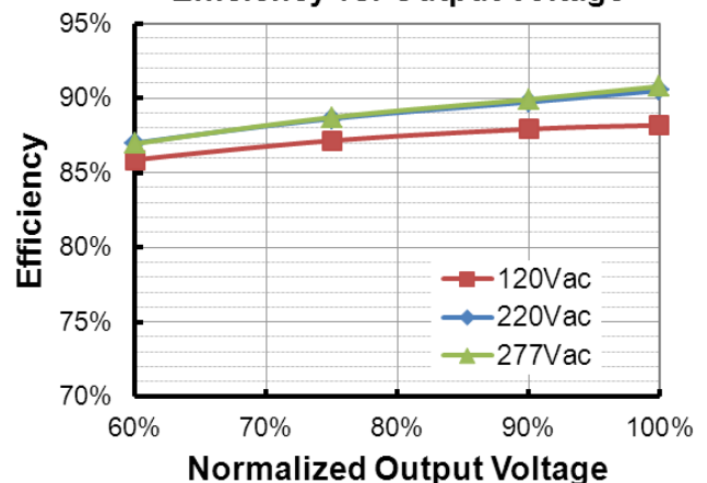
EUD-096S210DTL (I o =2100mA) Efficiency vs. Output Voltage
