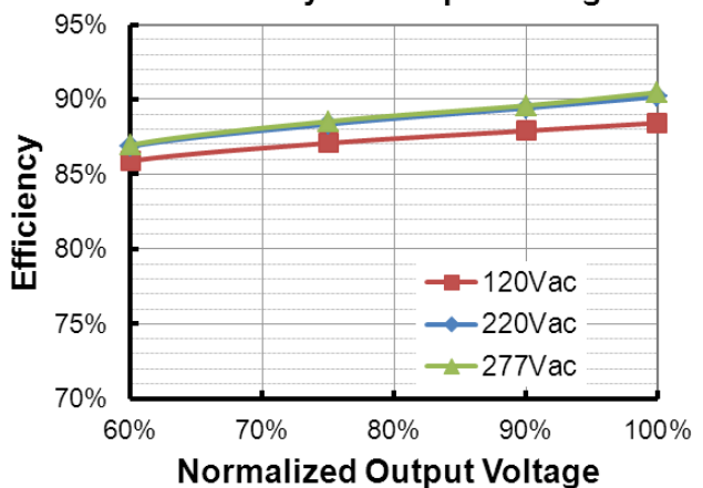
EUD-096S350DTL (Io=3500mA) Efficiency vs. Output Voltage
