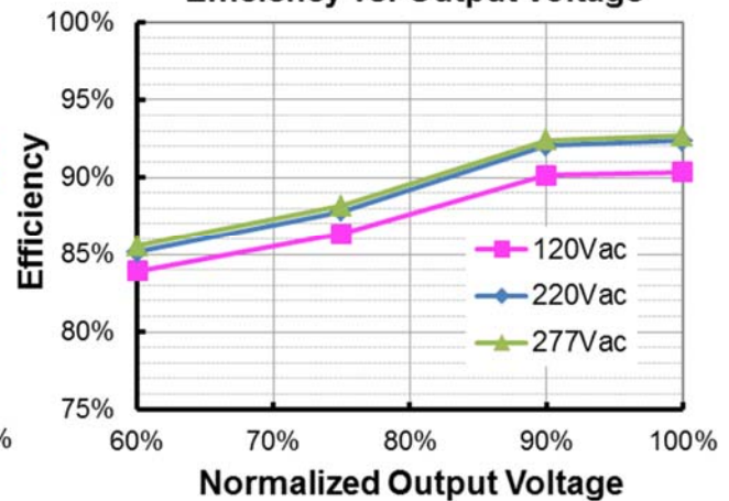
EUM-100S280Lx ( I_o=2800mA ) Efficiency vs. Output Voltage
