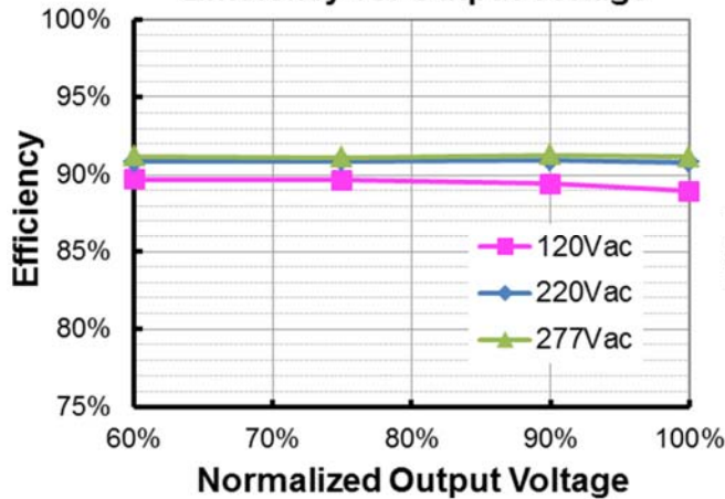
EUM-100S280Lx ( I_o=1750mA ) Efficiency vs. Output Voltage
