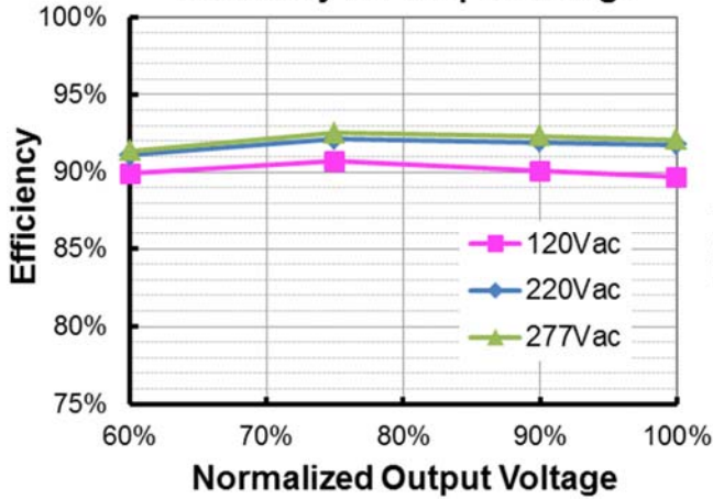
EUM-100S150Lx ( I_o=1050mA ) Efficiency vs. Output Voltage
