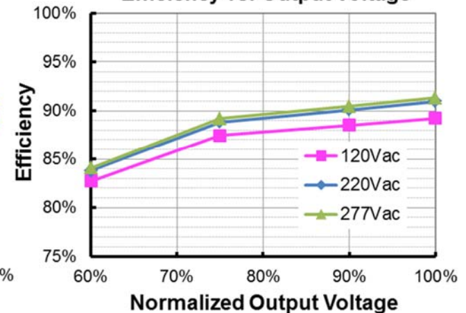
EUM-100S280Lx ( I_o=2800mA ) Efficiency vs. Output Voltage
