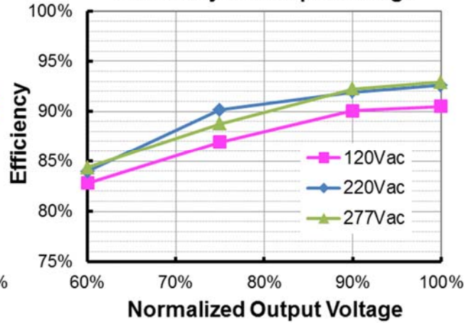
EUM-100S150Lx ( I_o=1500mA ) Efficiency vs. Output Voltage
