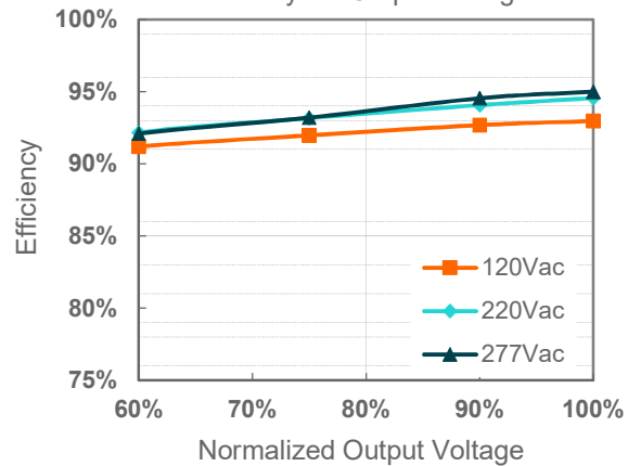
EUM-480S140Mx( I_o=1400mA ) Efficiency vs. Output Voltage
