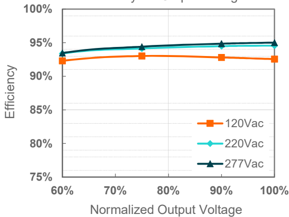
EUM-480S140Mx( I_o=1050mA ) Efficiency vs. Output Voltage
