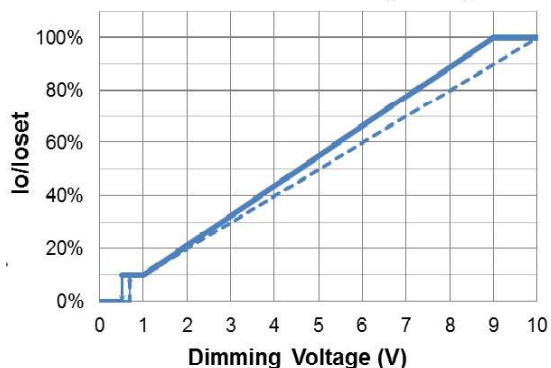
I_o/I_{o\text{set}} vs. Dimming Voltage
