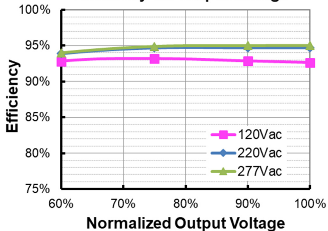
EUM-680S840Mx(Io=6300mA) Efficiency vs. Output Voltage
