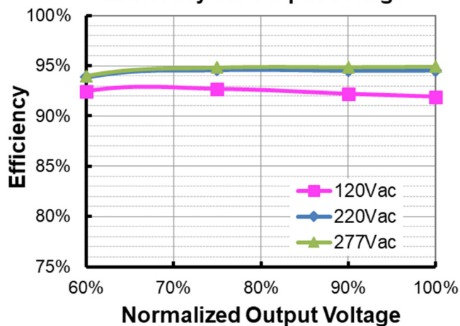
EUM-680S560Mx(Io=4200mA) Efficiency vs. Output Voltage
