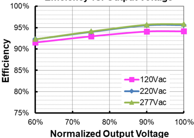
EUM-680S15AMx(Io=15000mA) Efficiency vs. Output Voltage
