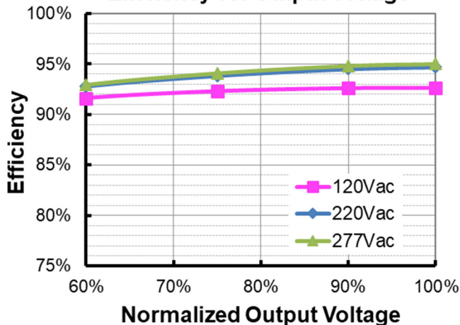
EUM-680S840Mx(Io=8400mA) Efficiency vs. Output Voltage
