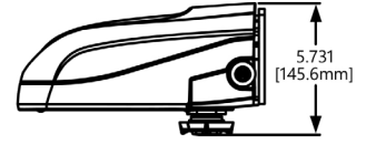
H Option - Wattstopper Motion Sensor Bottom mount available with A, B, C, D, & E Optical Codes Only
