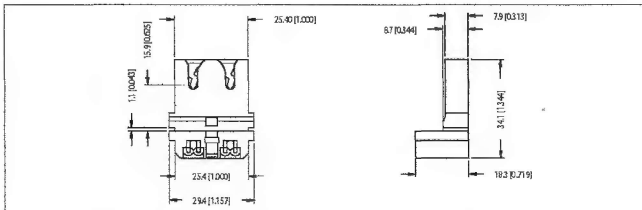
FL030 Solid Shoulders Slot Mount
