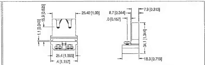
FL030-C Solid Shoulders Captive Nut Slot Mount
