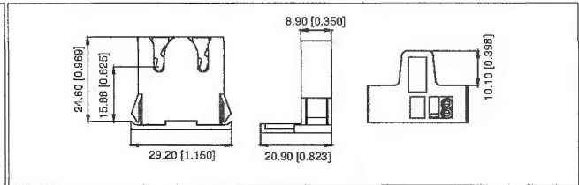
FL030-WS Flexible Snap-in Shoulders, Shunted
