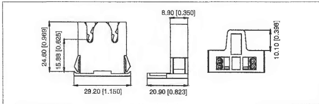
FL030-W Flexible Snap-in Shoulders
