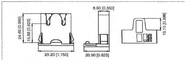
FL030-WSN Flexible Snap-in Shoulders, Shunted with Locating Nib
