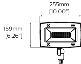
FL40-K Front
