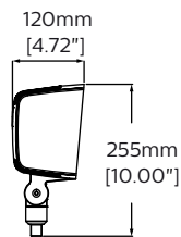
FL40-K Side
