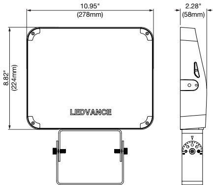
140W-TRUNNION
