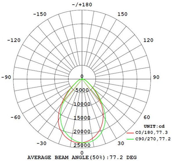
80° Optics Setting
