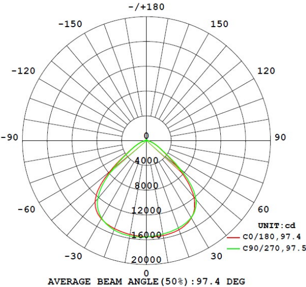
100° Optics Setting
