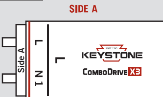
FIGURE C Direct Drive LED Tube Connection Pins
