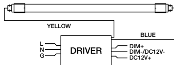
Wiring Diagram A
