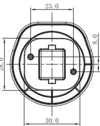
LEDlescent UL Type B Base – G24d
