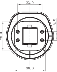
SubstiTUBE UL Type A Base – G24q
