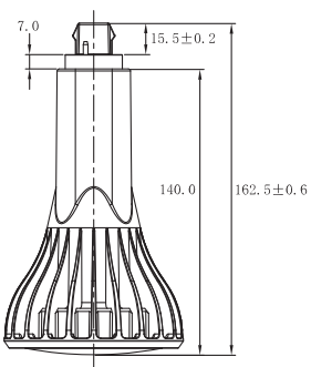
High Output UL Type B LEDlescent Vertical
