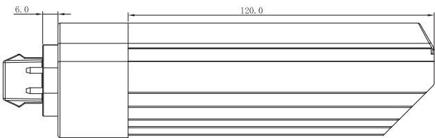
High Output UL Type B LEDlescent Horizontal
