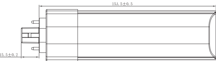
High Output UL Type A SubstiTUBE Horizontal
