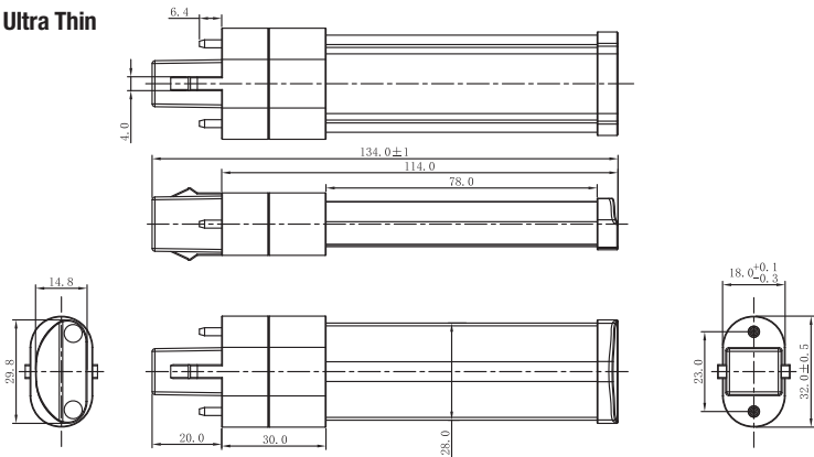
DUALescent™ Ultra Thin for GX23
