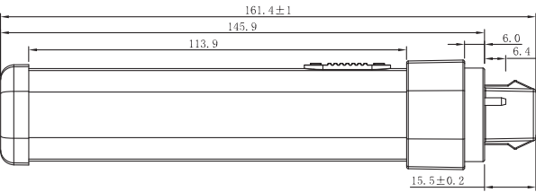
CCT Selectable UL Type A SubstiTUBE Horizontal
