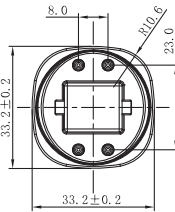
SubstiTUBE UL Type A Base – G24q
