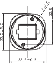
DUALescent UL Type A+B Base – G24d
