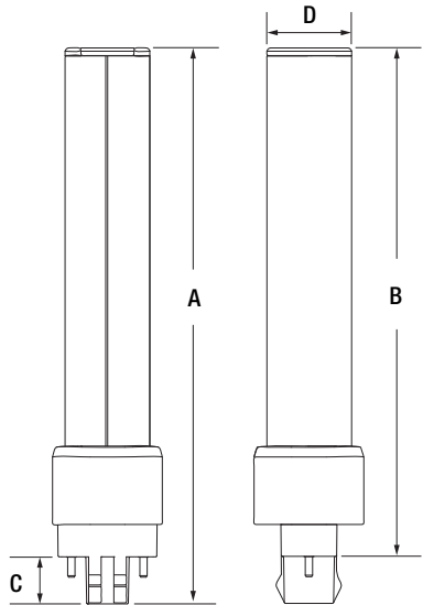
6W SubstiTUBE Base – GX23
