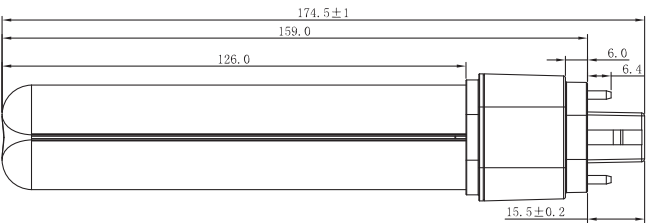
CCT Selectable UL Type A SubstiTUBE® and UL Type A+B DUALescent™ Horizontal
