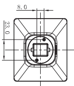
DUALescent UL Type A+B Base – G24d
