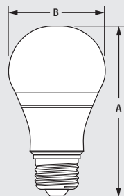
LED5.5 & LED9
