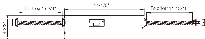
DIM010UNV or Fixed Output Driver
