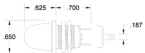
LHMF WITH DOME LENS
