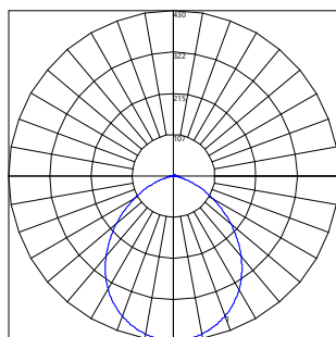
4" Square LRX 1000/650 Series LRXBS41X9WWVQ
