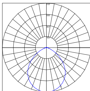
6" Square LRX 1800/1000/650 Series LRXBS61X9WWVQ
