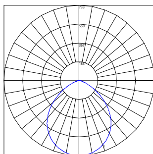
6" Round LRX 1800/1000/650 Series LRXBR61X9WWVQ
