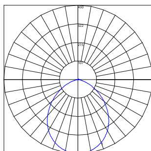
8" Round LRX 1800/1000/650 Series LRXBR81X9WWVQ
