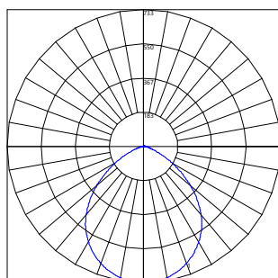
8" Square LRX 1800/1000/650 Series LRXBS81X9WWVQ
