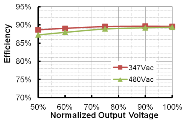
LTC-040S053DSP(SSP) Efficiency vs. Output Voltage
