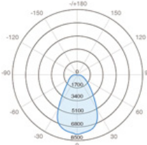
70° Reflector
