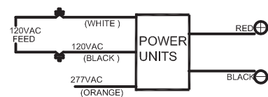
277V TAP CONNECTION
